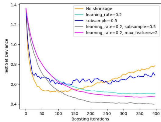
Fig 6.3: Model Training
